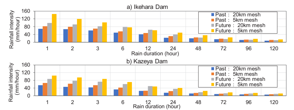
Fig. 8. Maximum rainfall intensity (maximum value) for each dam for the duration of rainfall in each case.
