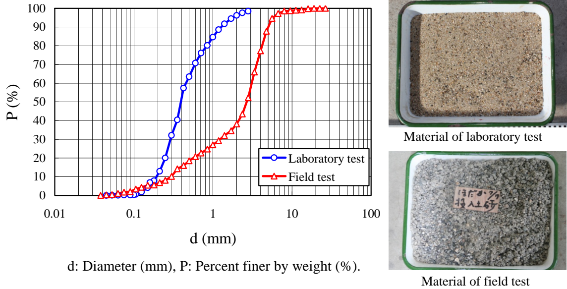
Figure 4. the Grain Size Distribution and the Photos of Sediment Materials.
