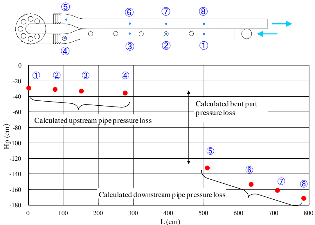
Figure 5. Example of Piezometric Head Profile.
