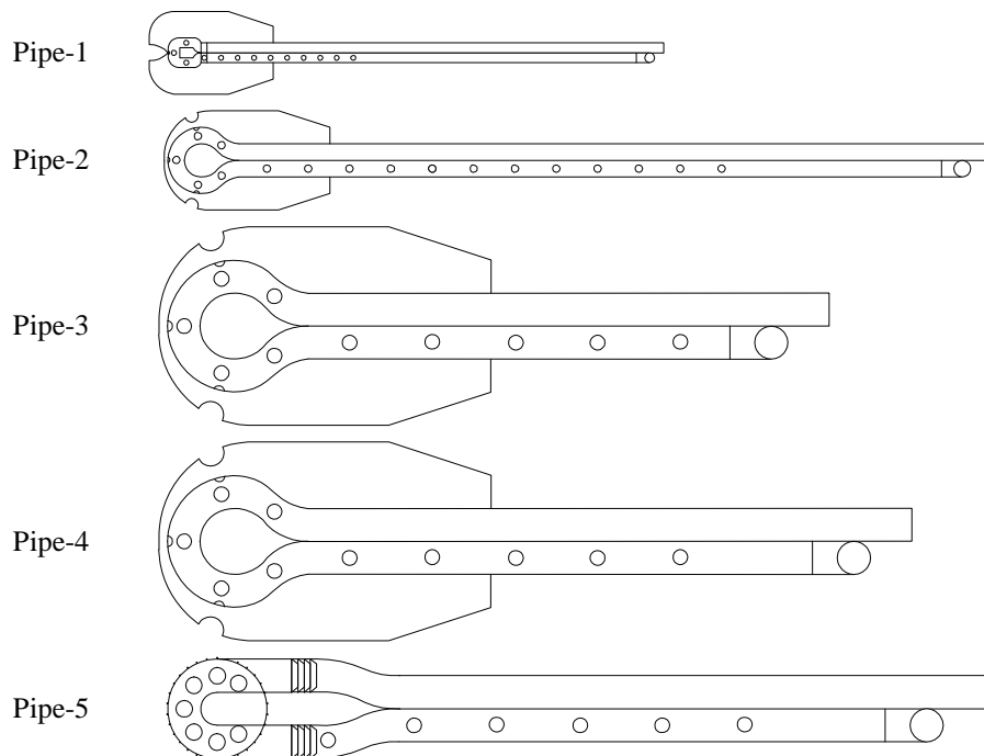
Figure 2. Plan View of the Suction Pipe Shapes.
