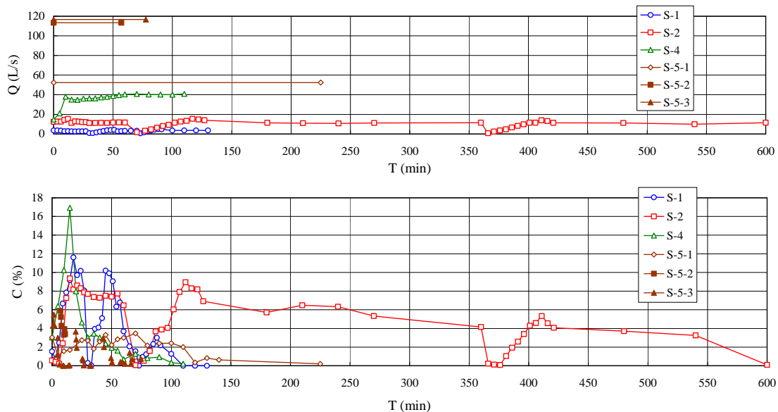
Figure 7. Time Series of Discharge Rate and Sediment Concentration.
