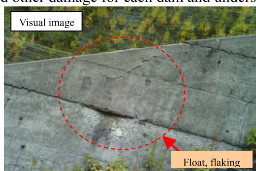
Figure 3: Image of visible concrete deterioration area
