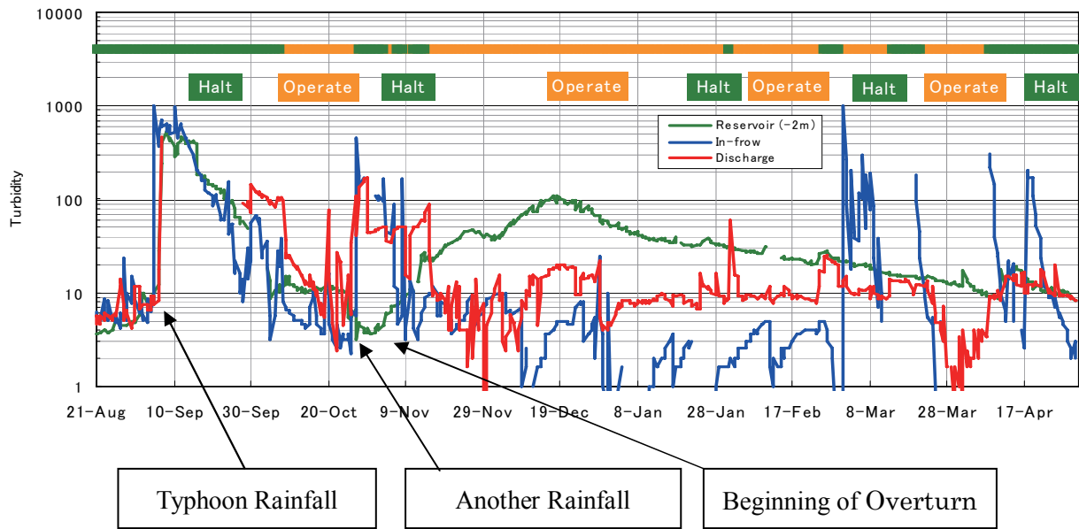
Fig.19 Inflow, Reservoir and Discharge Turbidity (NTU)
