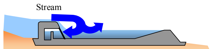
Fig.6 Cross-section of Intake
